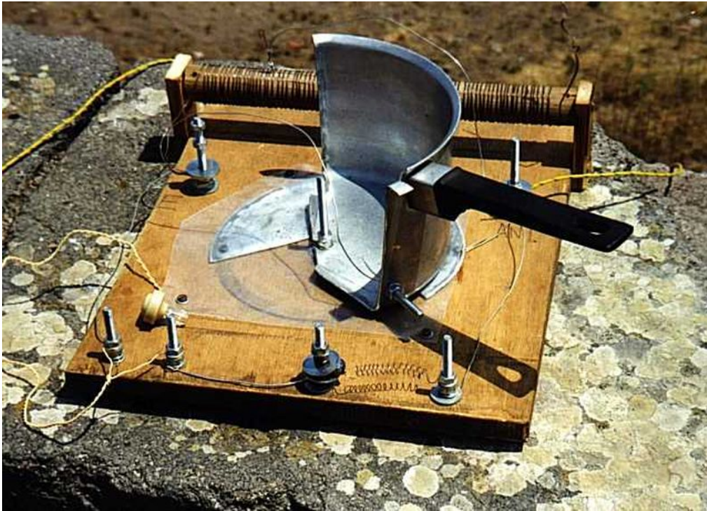
Figure 7: This will keep the tuning capacitor from cooking! Source: MBK
